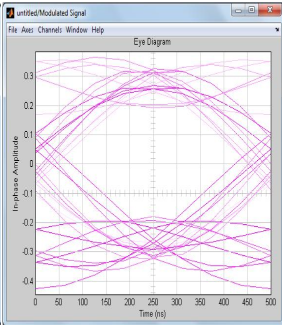
Modulated data displayed by discrete eye scope
