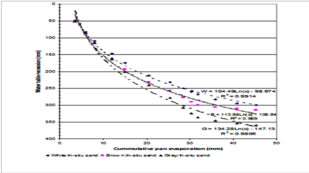
Figure 5: Effect of cumulative evaporation on water table recession: case of different colours of in situ sand
